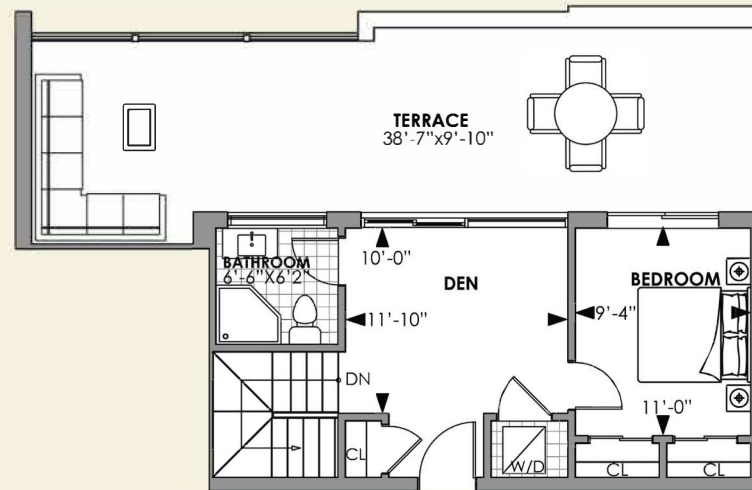
ROOF TOP TERRACE / PENTHOUSE
